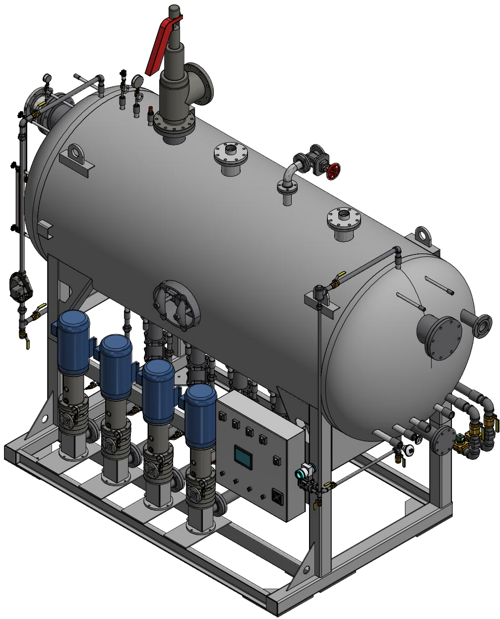
FRONT ISO VIEW
