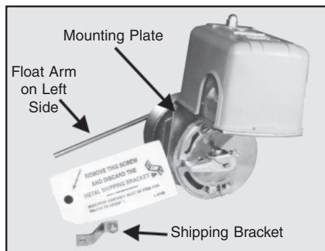
FIGURE 3—Float Switch
