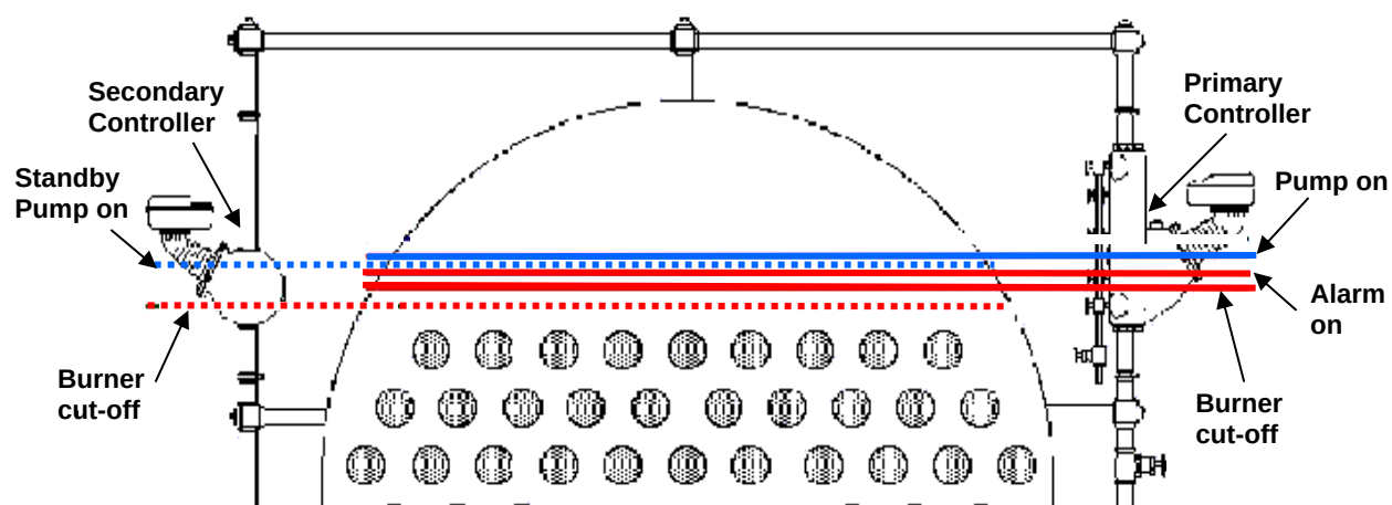
FIGURE 2 TWO COMBINATION CONTROLLERS FOR BOILER FEED STANDBY
